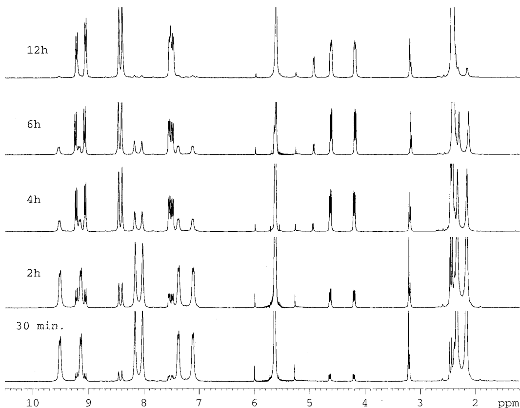
Figure 2. ^1\text{H} NMR follow-up experiment of the reaction between 3 and dichloromethane in [\text{D}_6]\text{DMSO}
