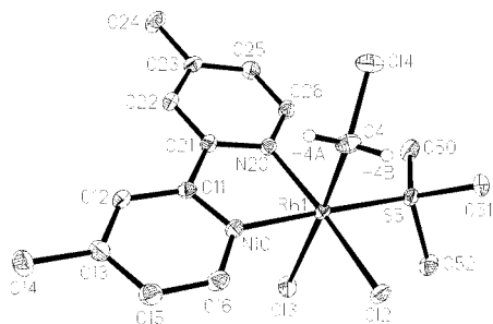
Figure 3. ORTEP drawing of a molecule of 8 (50% of probability); hydrogen atoms (except Rh-CH_2Cl ) are omitted for clarity
