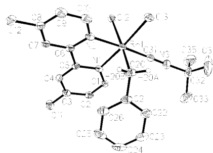
Figure 4. ORTEP drawing of a molecule of 9 (50% of probability); hydrogen atoms (except Rh-CH_2R ) are omitted for clarity
