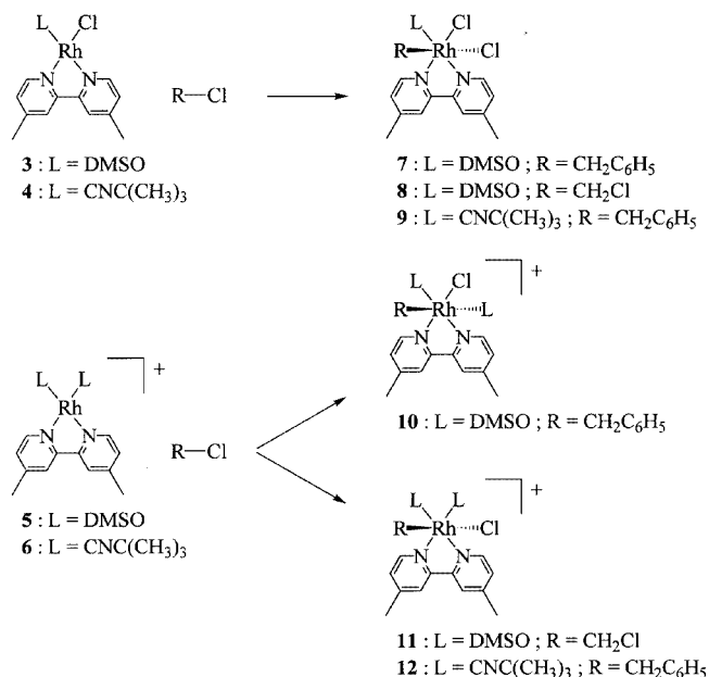
Scheme 3. Reaction of the \text{Rh}^{\text{I}} complexes 3–6 with \text{R–Cl} to yield the \text{Rh}^{\text{III}} complexes 7–12
