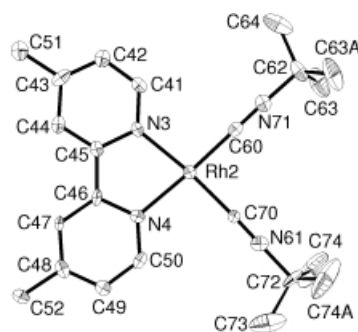
Figure 1. ORTEP drawing of a molecule of 6 (50% of probability); hydrogen atoms are omitted for clarity
