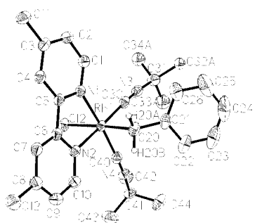
Figure 5. ORTEP drawing of a molecule of 12 (50% of probability); hydrogen atoms (except Rh–CH 2 R) are omitted for clarity
