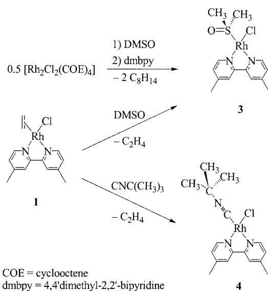
Scheme 1. Synthesis of the neutral \text{Rh}^{\text{I}} complexes 3 and 4
