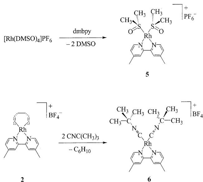
Scheme 2. Synthesis of the cationic \text{Rh}^{\text{I}} complexes 5 and 6
