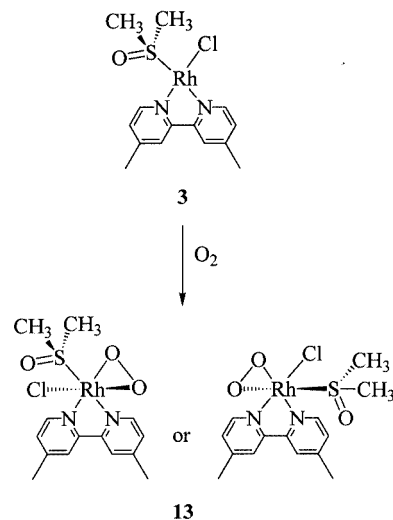
Scheme 4. Reaction of complex 3 with O 2 giving the peroxo complex 13
